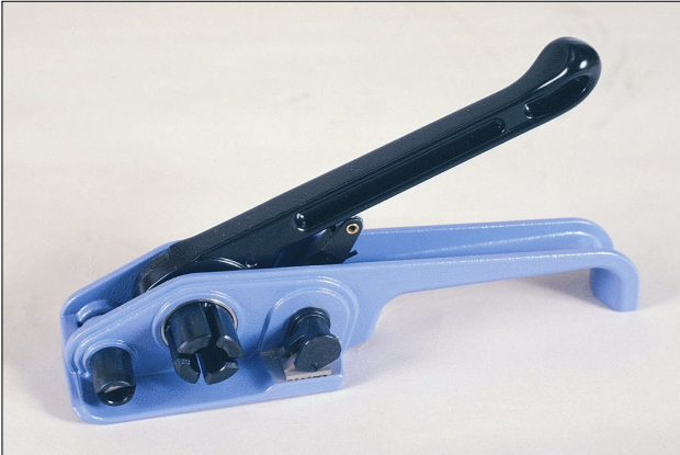
PT34W Tensioner – Code T7918A Budget Tensioner for Poly strap 12-19mm No spare parts available
